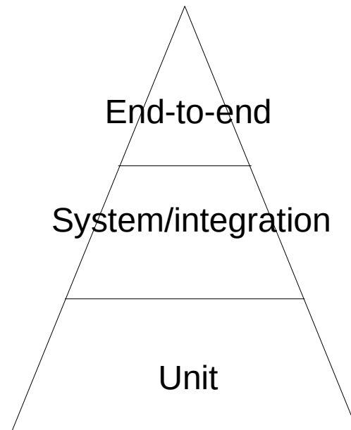
Testing pyramid
